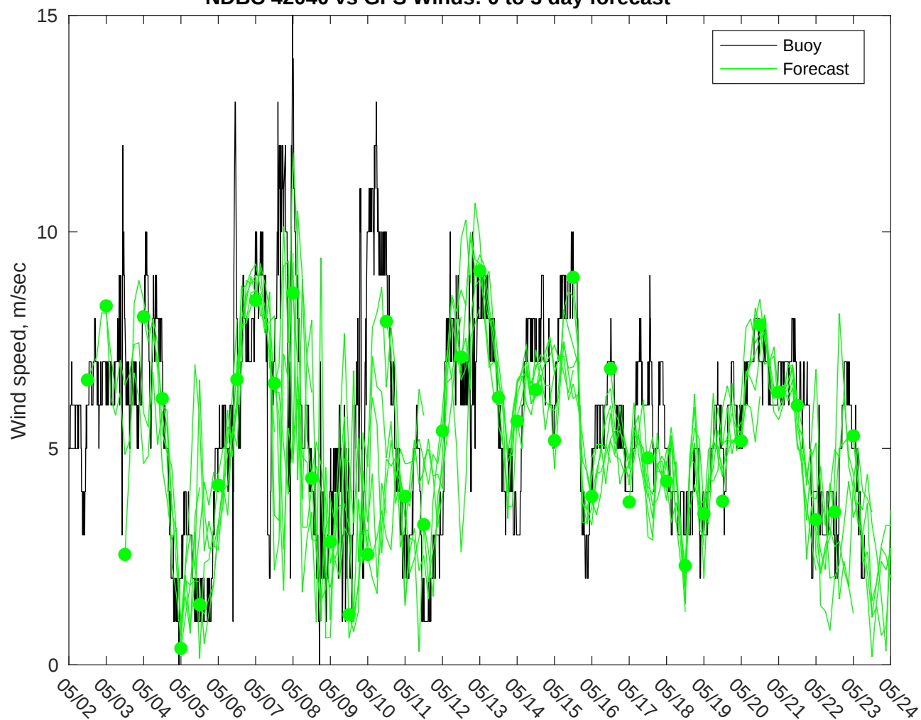
NDBC 42040 vs GFS Winds: 0 to 3 day forecast
