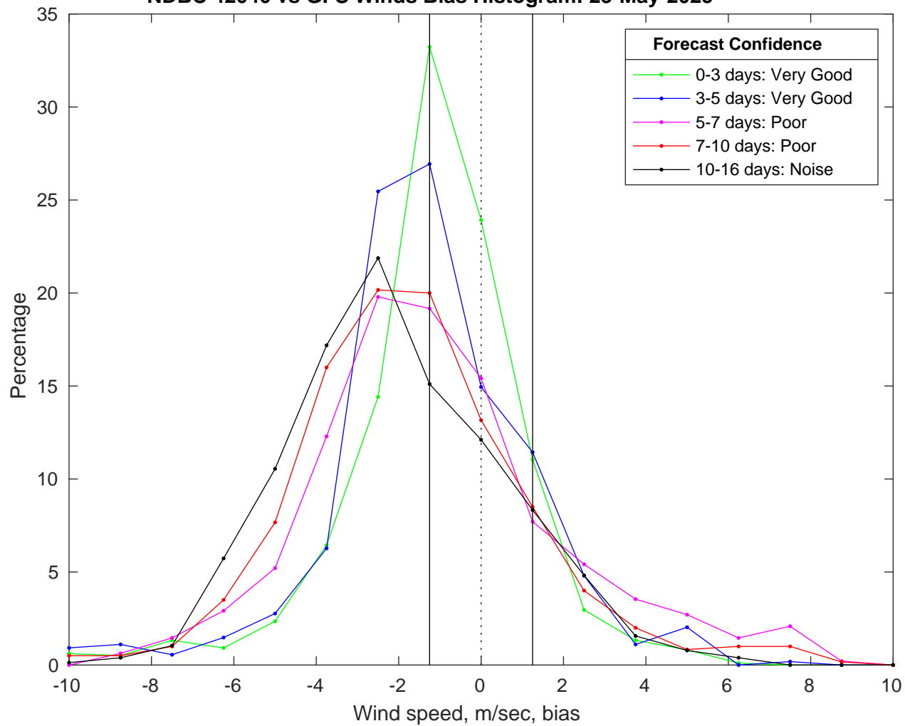
NDBC 42040 vs GFS Winds Bias Histogram: 23-May-2025
