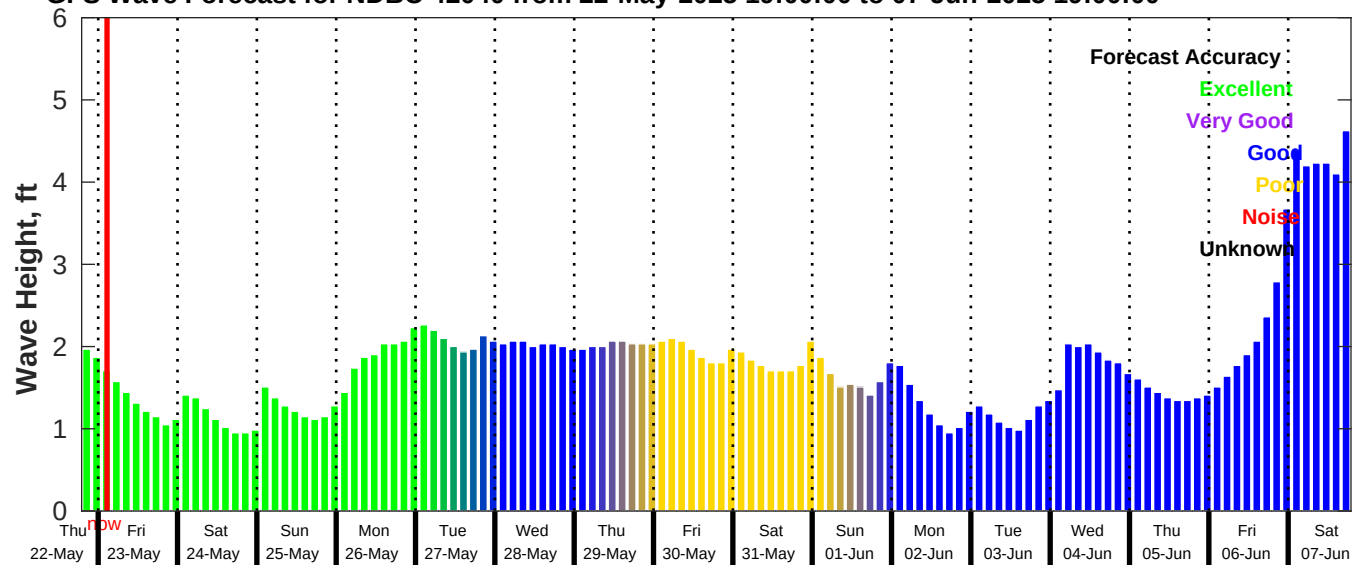
GFS Wave Forecast for NDBC 42040 from 22-May-2025 19:00:00 to 07-Jun-2025 19:00:00
