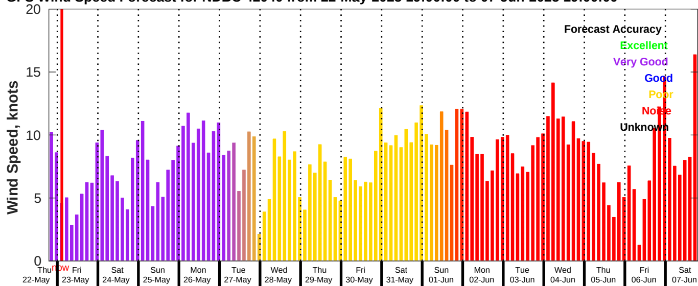
GFS Wind Speed Forecast for NDBC 42040 from 22-May-2025 19:00:00 to 07-Jun-2025 19:00:00
