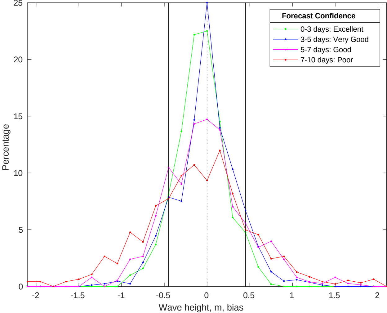
NDBC 46011 vs CMEMS Waves Bias Histogram: 23-May-2025
