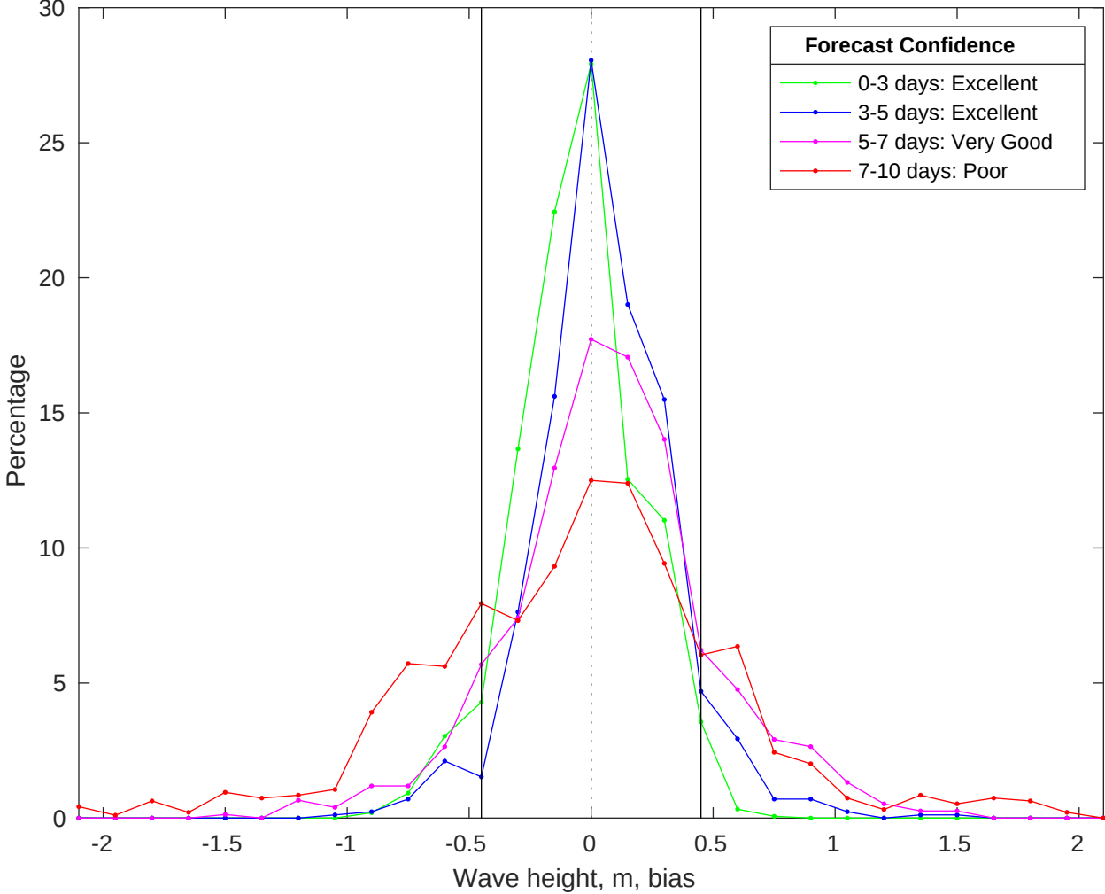
NDBC 46028 vs CMEMS Waves Bias Histogram: 23-May-2025
