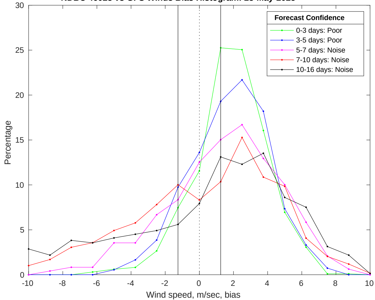
NDBC 46028 vs GFS Winds Bias Histogram: 23-May-2025
