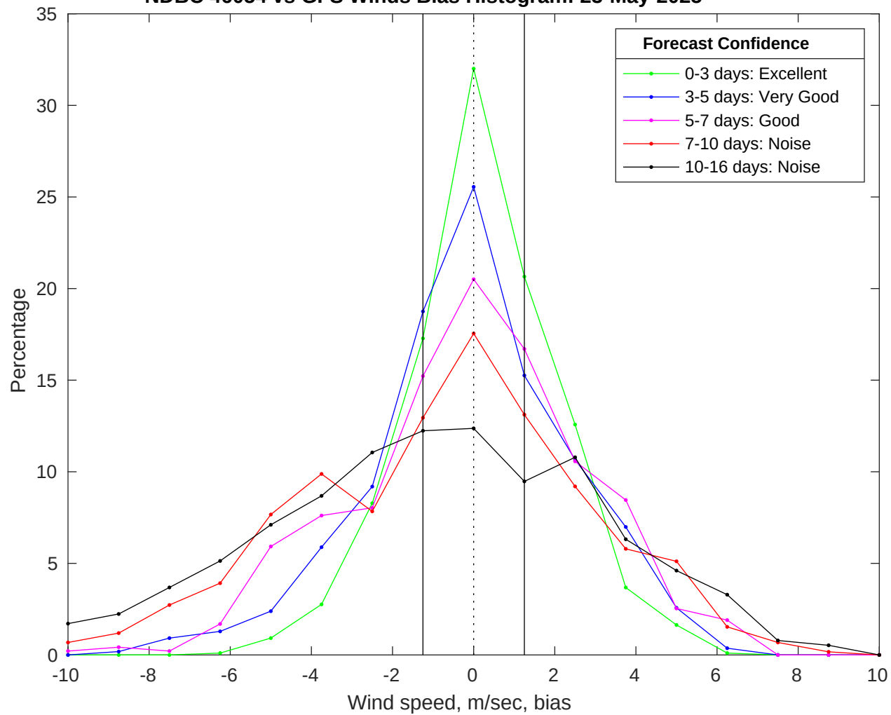
NDBC 46054 vs GFS Winds Bias Histogram: 23-May-2025
