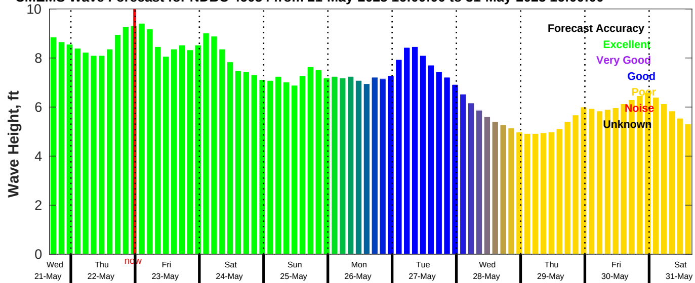
CMEMS Wave Forecast for NDBC 46054 from 21-May-2025 16:00:00 to 31-May-2025 16:00:00
