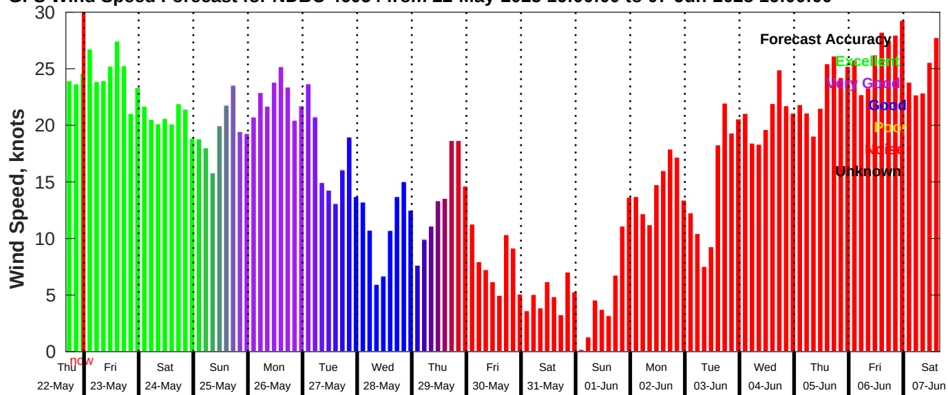
GFS Wind Speed Forecast for NDBC 46054 from 22-May-2025 16:00:00 to 07-Jun-2025 16:00:00
