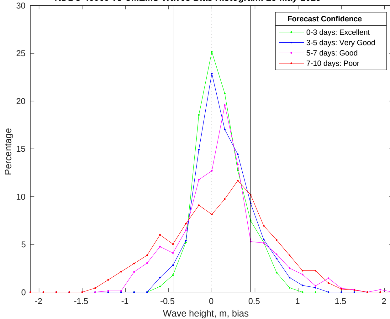
NDBC 46069 vs CMEMS Waves Bias Histogram: 23-May-2025
