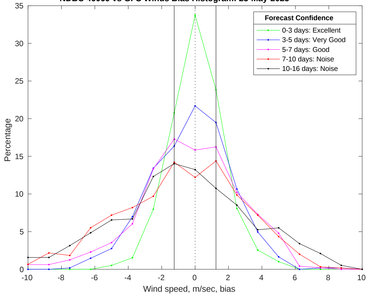
NDBC 46069 vs GFS Winds Bias Histogram: 23-May-2025
