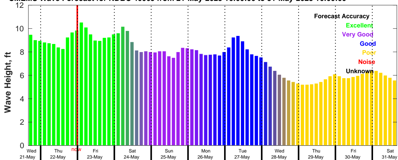
CMEMS Wave Forecast for NDBC 46069 from 21-May-2025 16:00:00 to 31-May-2025 16:00:00
