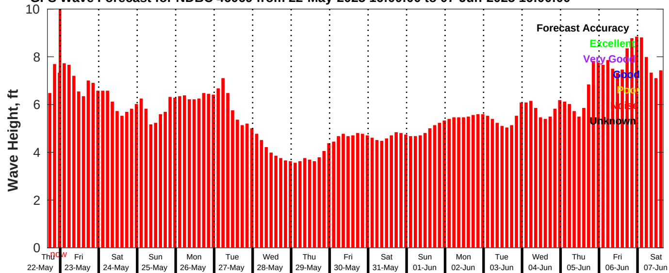
GFS Wave Forecast for NDBC 46069 from 22-May-2025 16:00:00 to 07-Jun-2025 16:00:00
