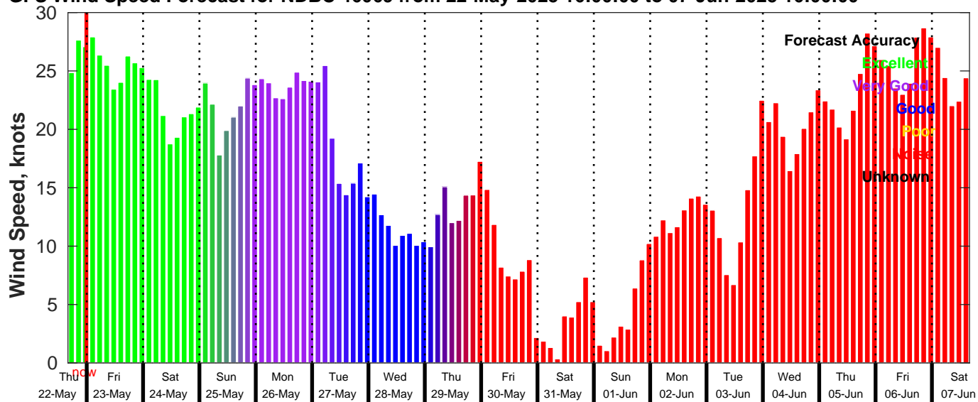
GFS Wind Speed Forecast for NDBC 46069 from 22-May-2025 16:00:00 to 07-Jun-2025 16:00:00
