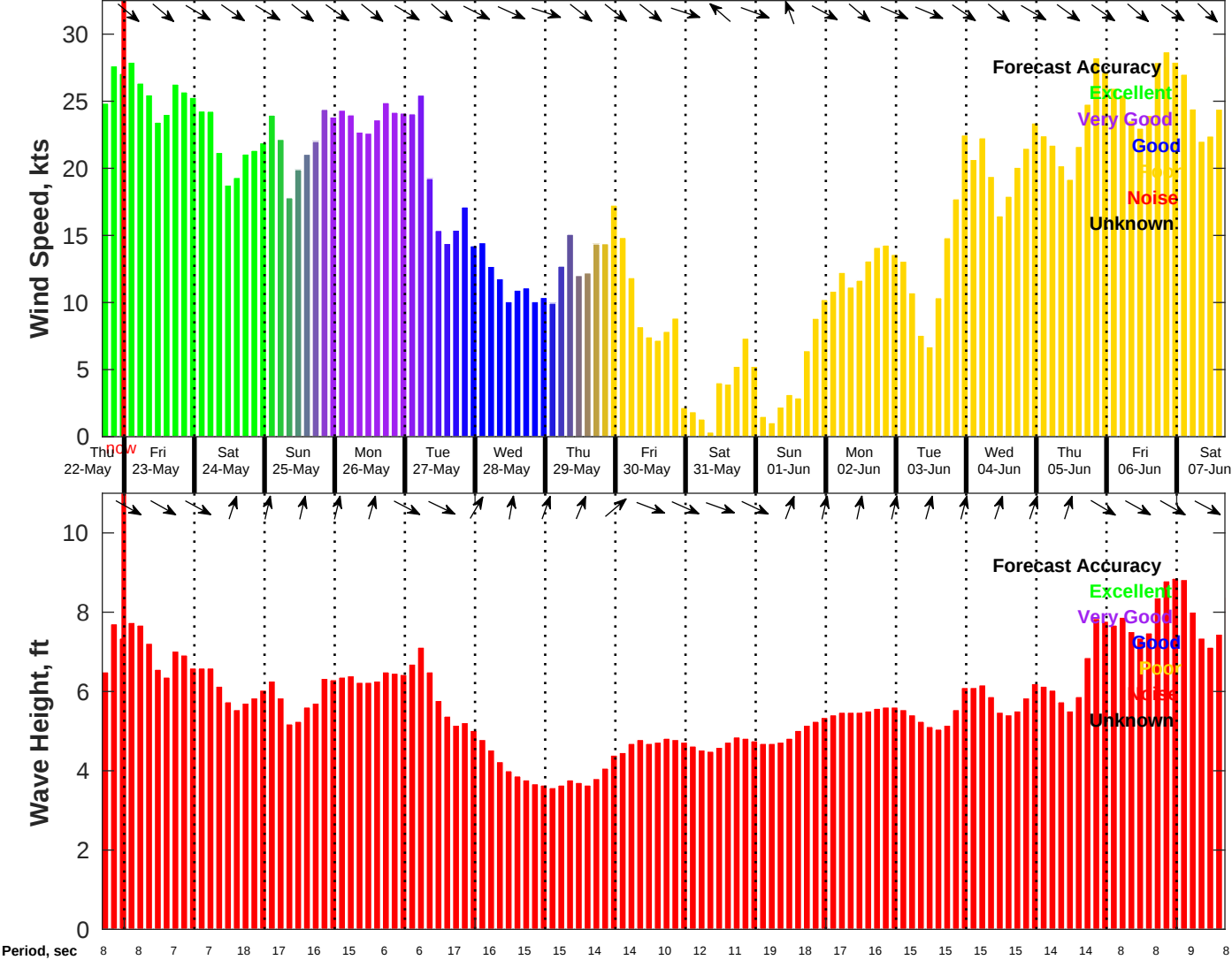
Wind & Wave Forecast for NDBC 46069 from 22-May-2025 16:00:00 to 07-Jun-2025 16:00:00
