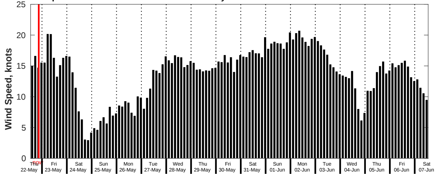
GFS Wind Speed Forecast for NDBC 51209 from 22-May-2025 13:00:00 to 07-Jun-2025 13:00:00
