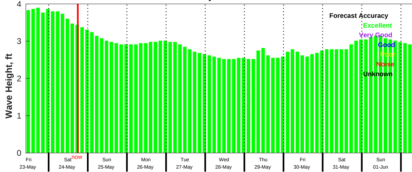
CMEMS Wave Forecast for NDBC 52211 from 22-May-2025 10:00:00 to 01-Jun-2025 10:00:00
