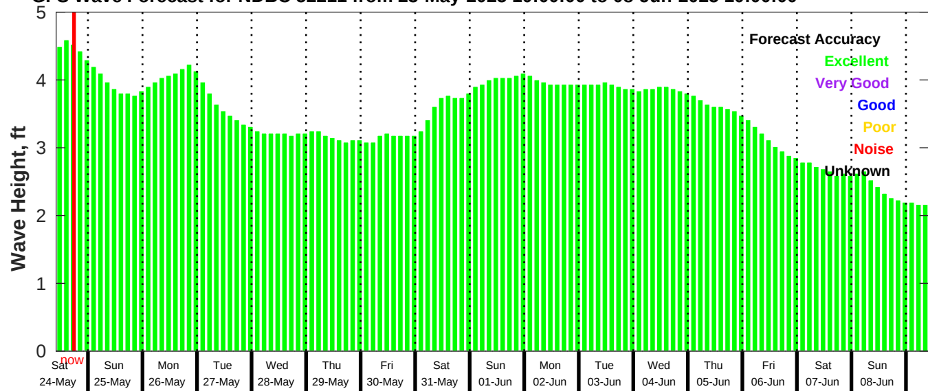
GFS Wave Forecast for NDBC 52211 from 23-May-2025 10:00:00 to 08-Jun-2025 10:00:00
