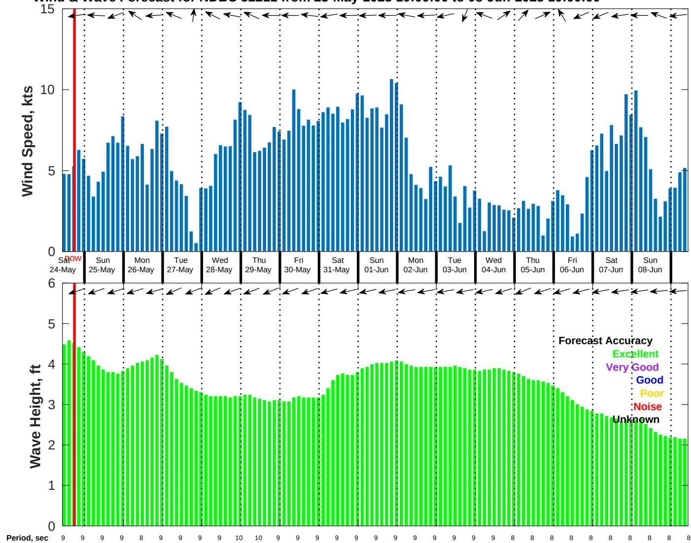
Wind & Wave Forecast for NDBC 52211 from 23-May-2025 10:00:00 to 08-Jun-2025 10:00:00
