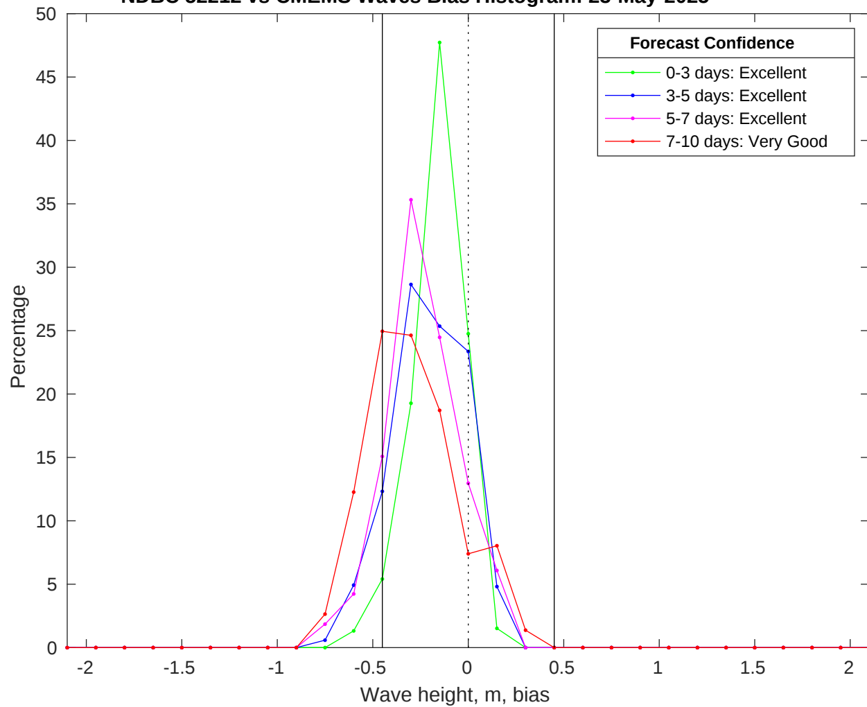
NDBC 52212 vs CMEMS Waves Bias Histogram: 23-May-2025
