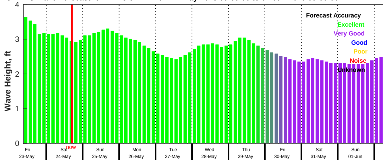
CMEMS Wave Forecast for NDBC 52212 from 22-May-2025 09:00:00 to 01-Jun-2025 09:00:00
