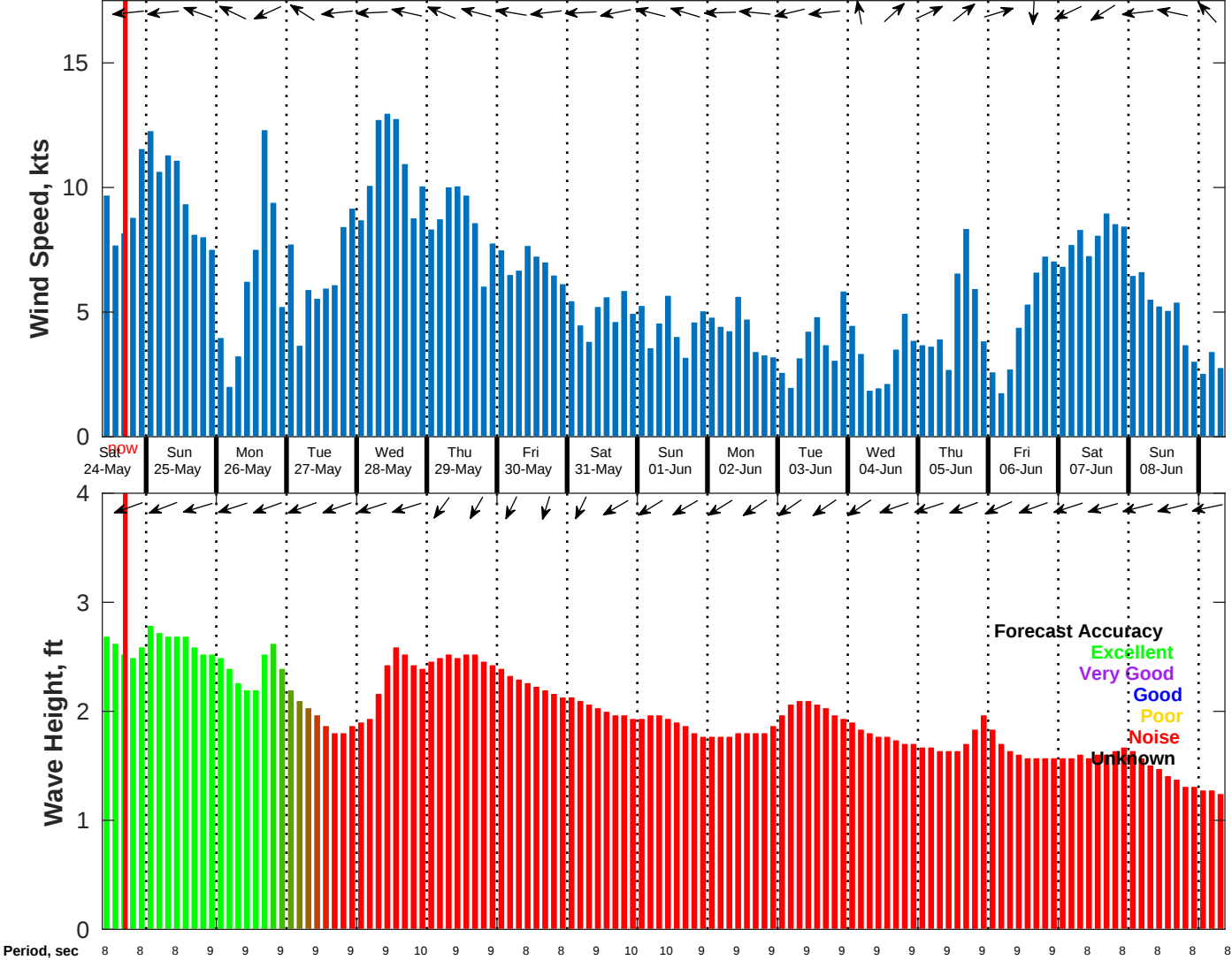
Wind & Wave Forecast for NDBC 52212 from 23-May-2025 09:00:00 to 08-Jun-2025 09:00:00
