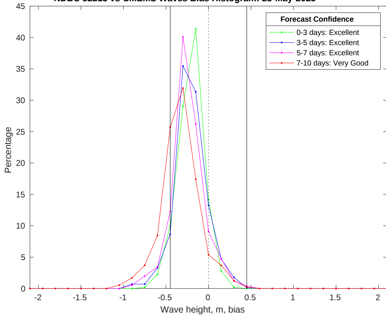
NDBC 52213 vs CMEMS Waves Bias Histogram: 23-May-2025
