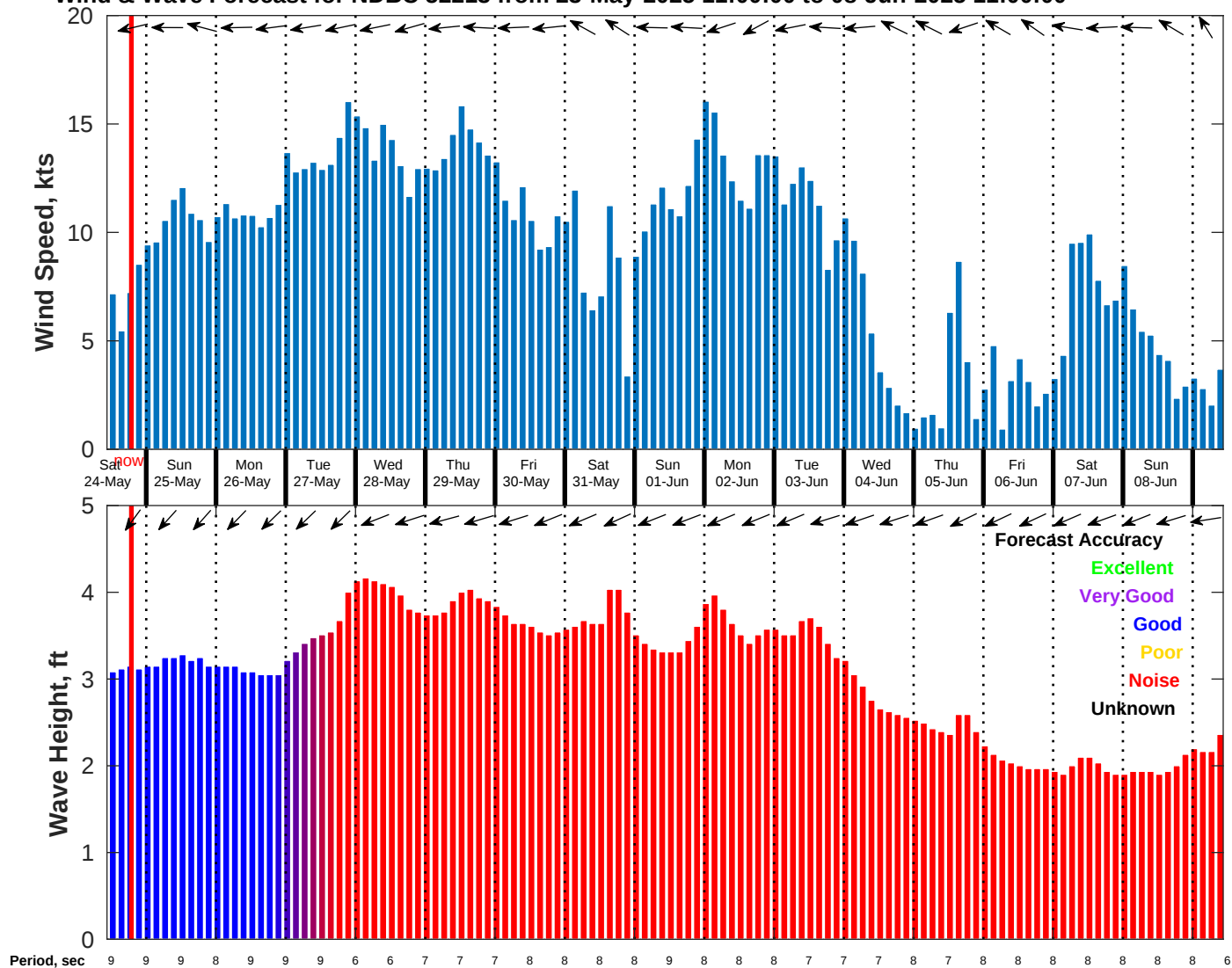
Wind & Wave Forecast for NDBC 52213 from 23-May-2025 11:00:00 to 08-Jun-2025 11:00:00
