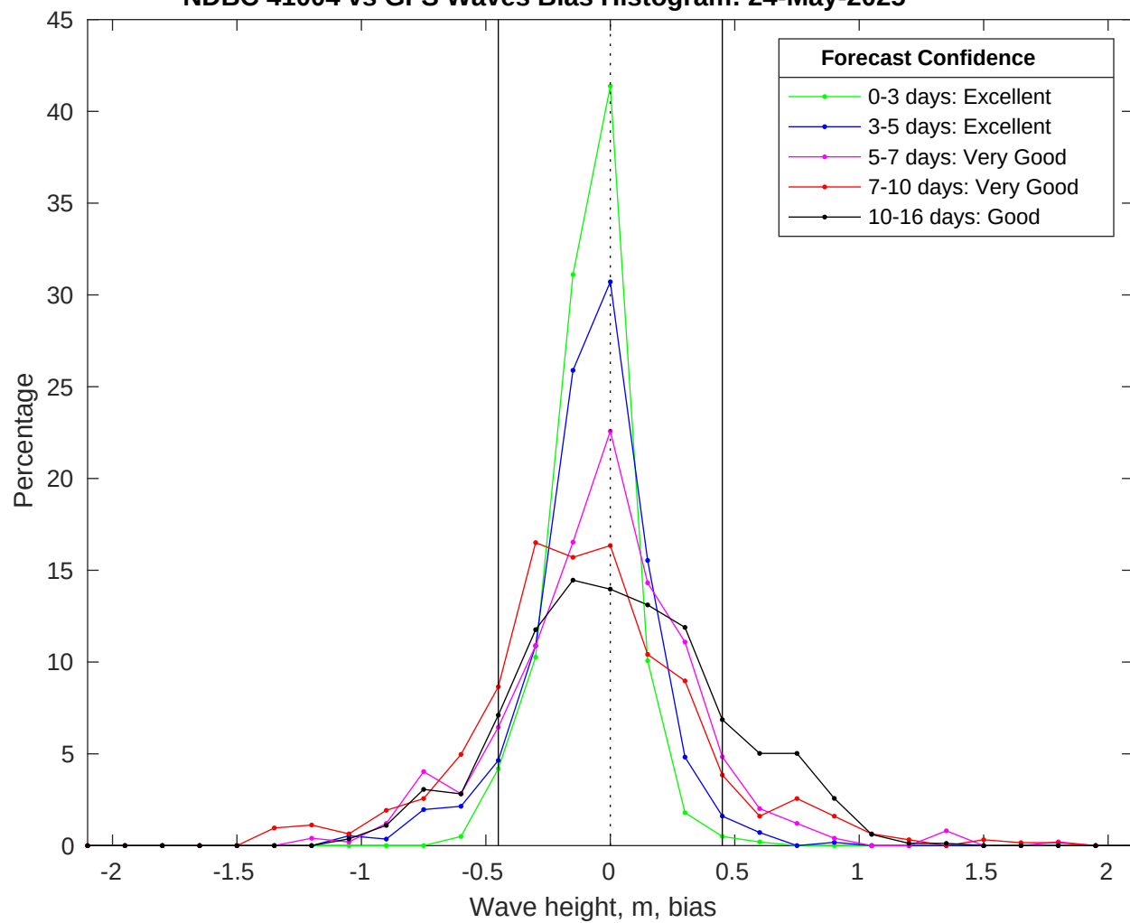
NDBC 41004 vs GFS Waves Bias Histogram: 24-May-2025
