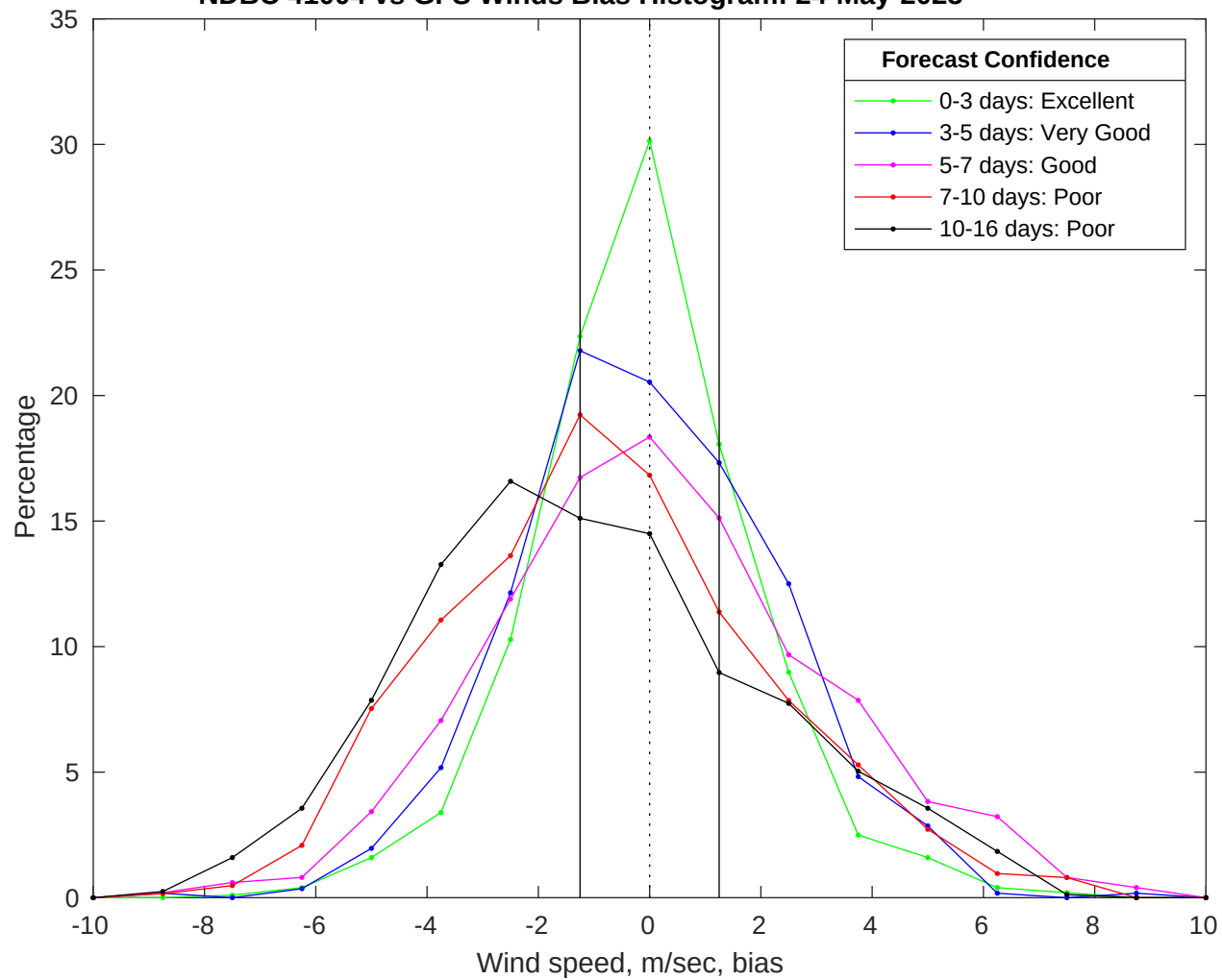
NDBC 41004 vs GFS Winds Bias Histogram: 24-May-2025
