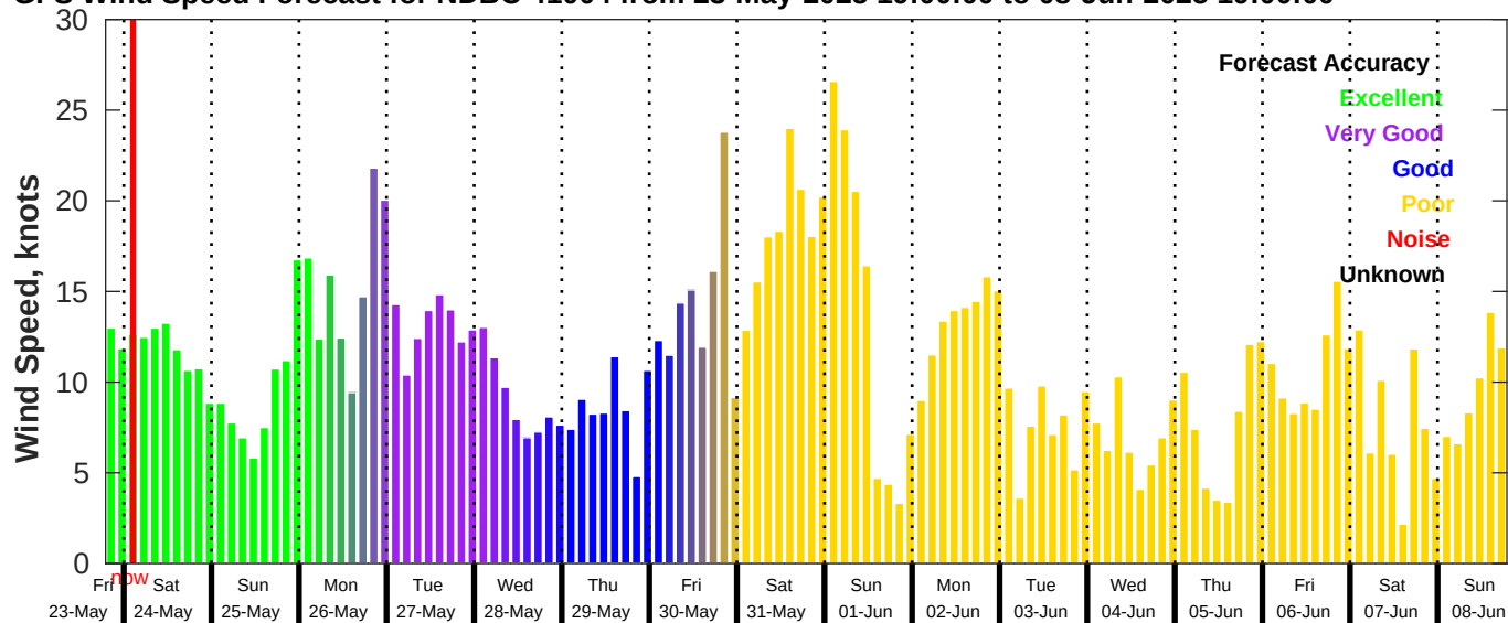
GFS Wind Speed Forecast for NDBC 41004 from 23-May-2025 19:00:00 to 08-Jun-2025 19:00:00
