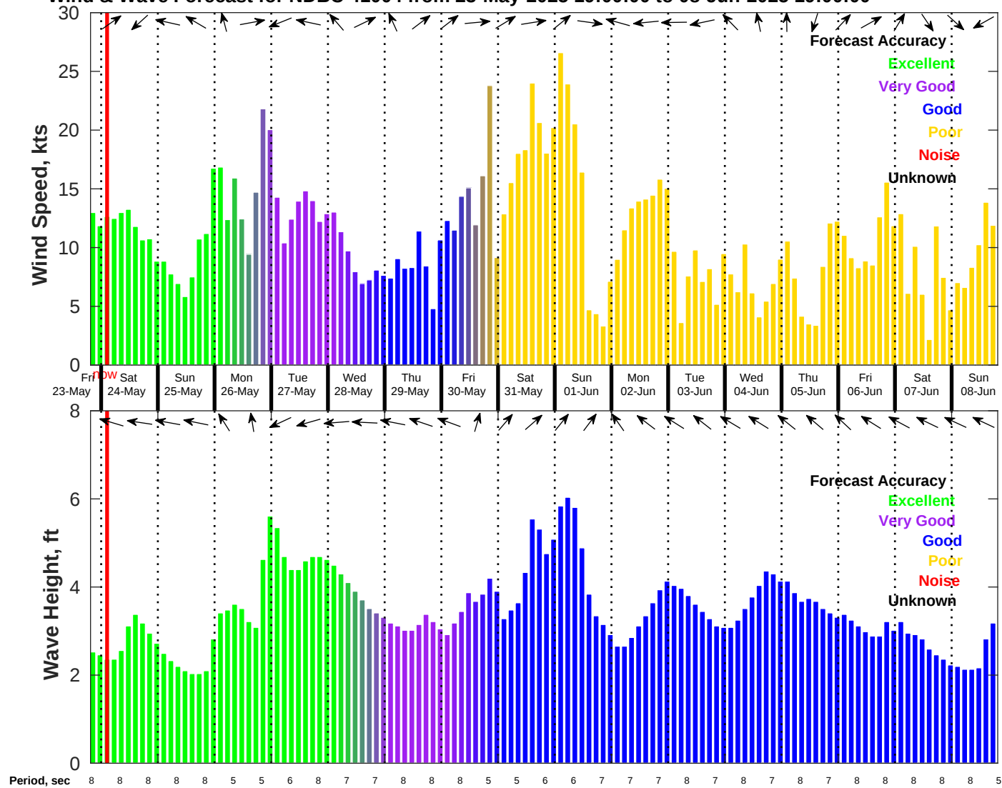
Wind & Wave Forecast for NDBC 41004 from 23-May-2025 19:00:00 to 08-Jun-2025 19:00:00
