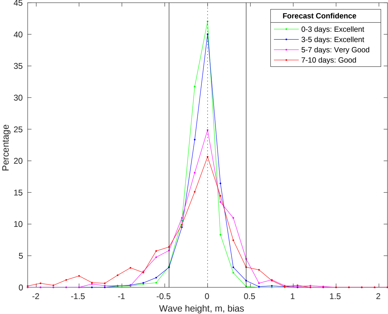
NDBC 41013 vs CMEMS Waves Bias Histogram: 24-May-2025
