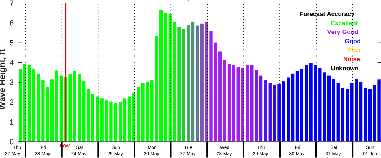
CMEMS Wave Forecast for NDBC 41013 from 22-May-2025 19:00:00 to 01-Jun-2025 19:00:00
