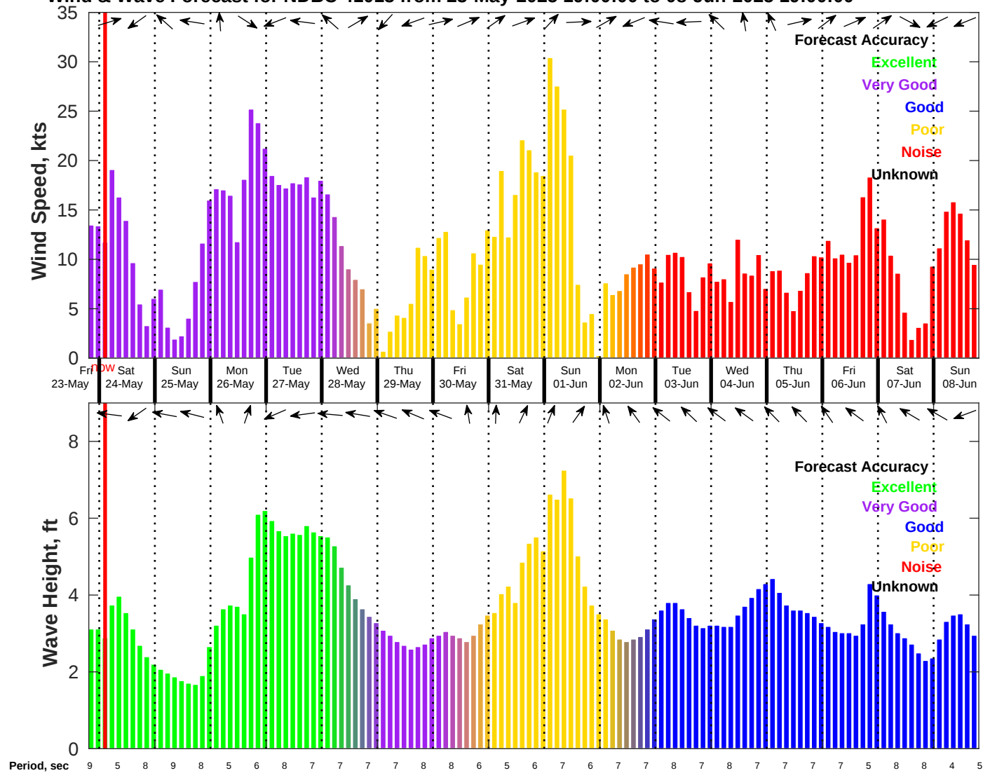
Wind & Wave Forecast for NDBC 41013 from 23-May-2025 19:00:00 to 08-Jun-2025 19:00:00
