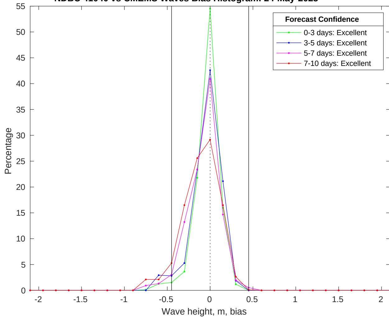
NDBC 41040 vs CMEMS Waves Bias Histogram: 24-May-2025
