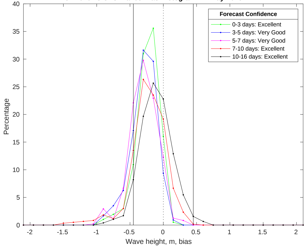
NDBC 41040 vs GFS Waves Bias Histogram: 24-May-2025
