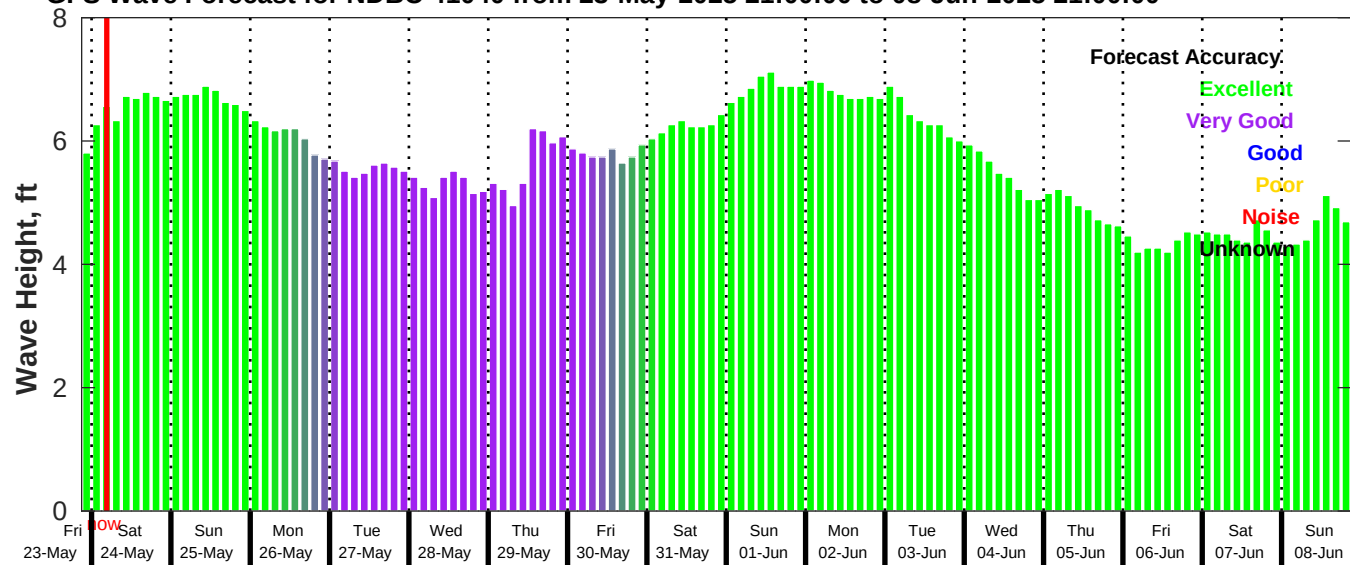
GFS Wave Forecast for NDBC 41040 from 23-May-2025 21:00:00 to 08-Jun-2025 21:00:00
