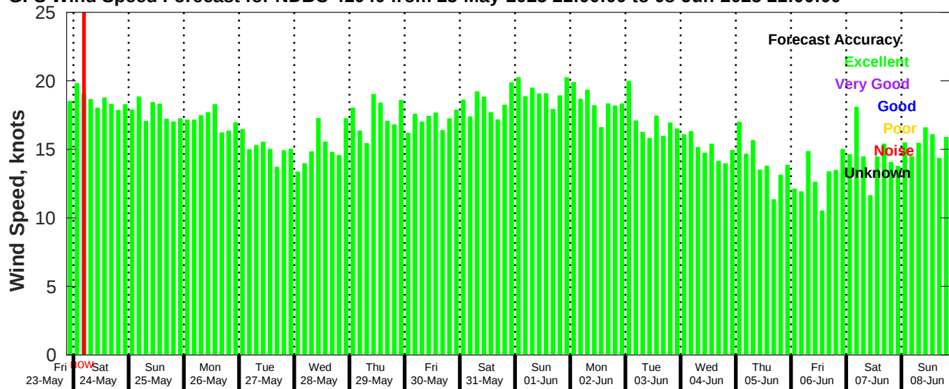
GFS Wind Speed Forecast for NDBC 41040 from 23-May-2025 21:00:00 to 08-Jun-2025 21:00:00
