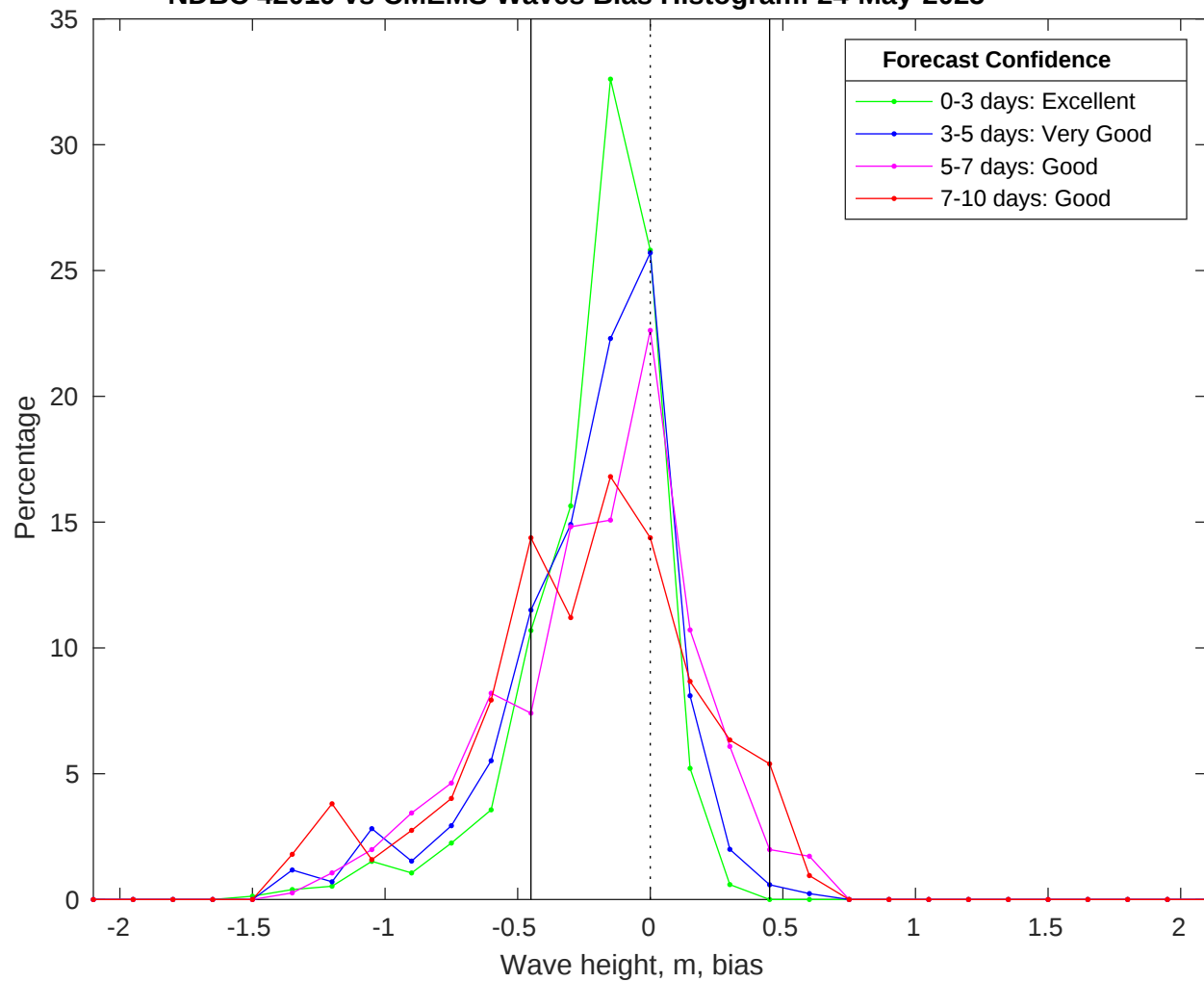
NDBC 42019 vs CMEMS Waves Bias Histogram: 24-May-2025
