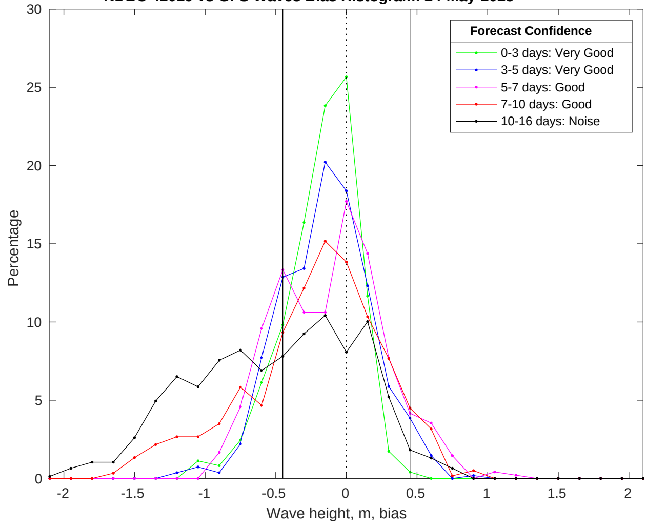
NDBC 42019 vs GFS Waves Bias Histogram: 24-May-2025
