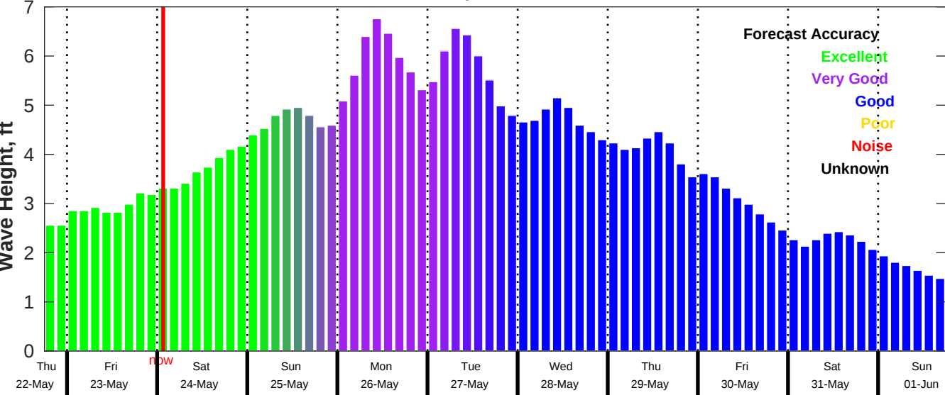
CMEMS Wave Forecast for NDBC 42019 from 22-May-2025 18:00:00 to 01-Jun-2025 18:00:00
