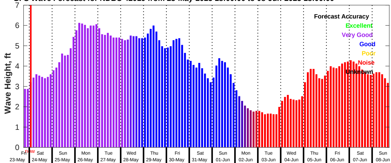
GFS Wave Forecast for NDBC 42019 from 23-May-2025 18:00:00 to 08-Jun-2025 18:00:00
