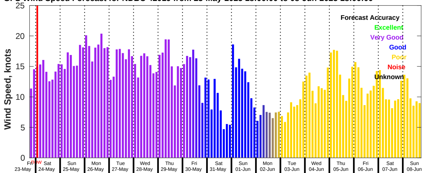
GFS Wind Speed Forecast for NDBC 42019 from 23-May-2025 18:00:00 to 08-Jun-2025 18:00:00
