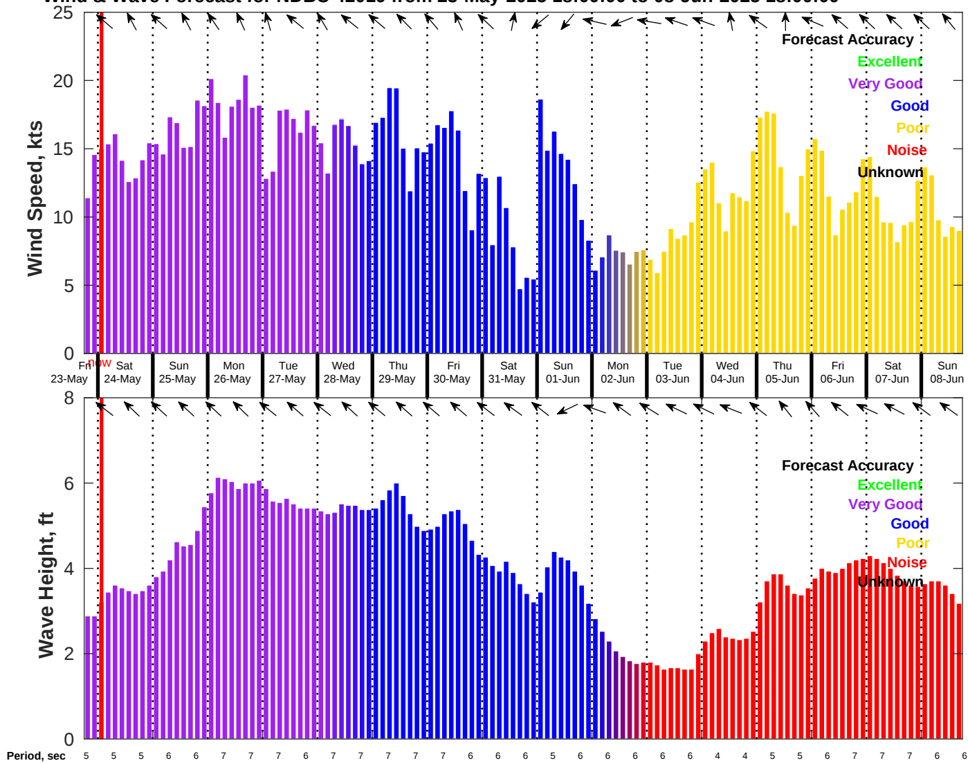
Wind & Wave Forecast for NDBC 42019 from 23-May-2025 18:00:00 to 08-Jun-2025 18:00:00
