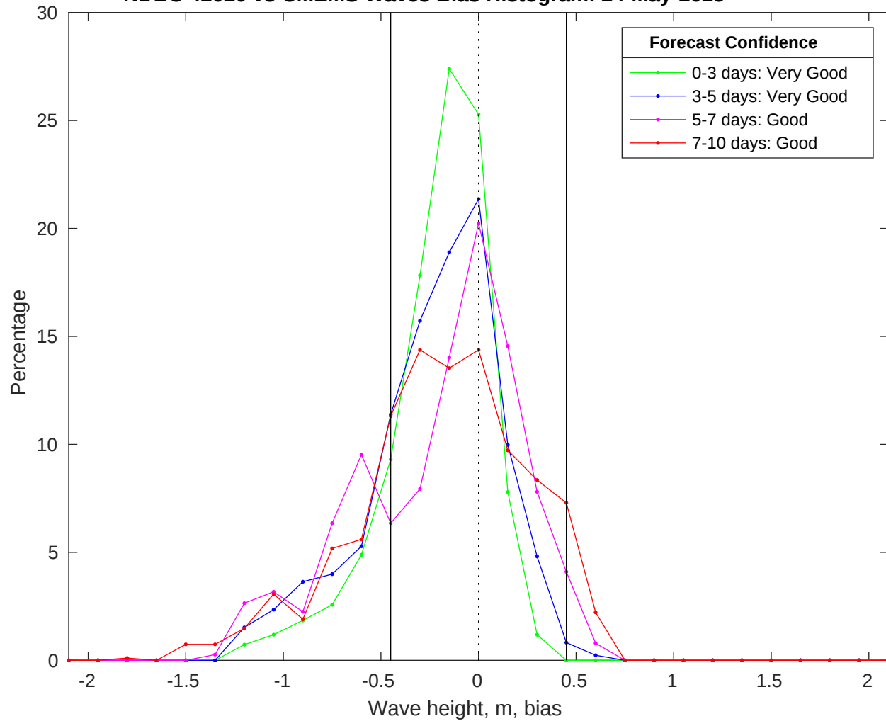
NDBC 42020 vs CMEMS Waves Bias Histogram: 24-May-2025
