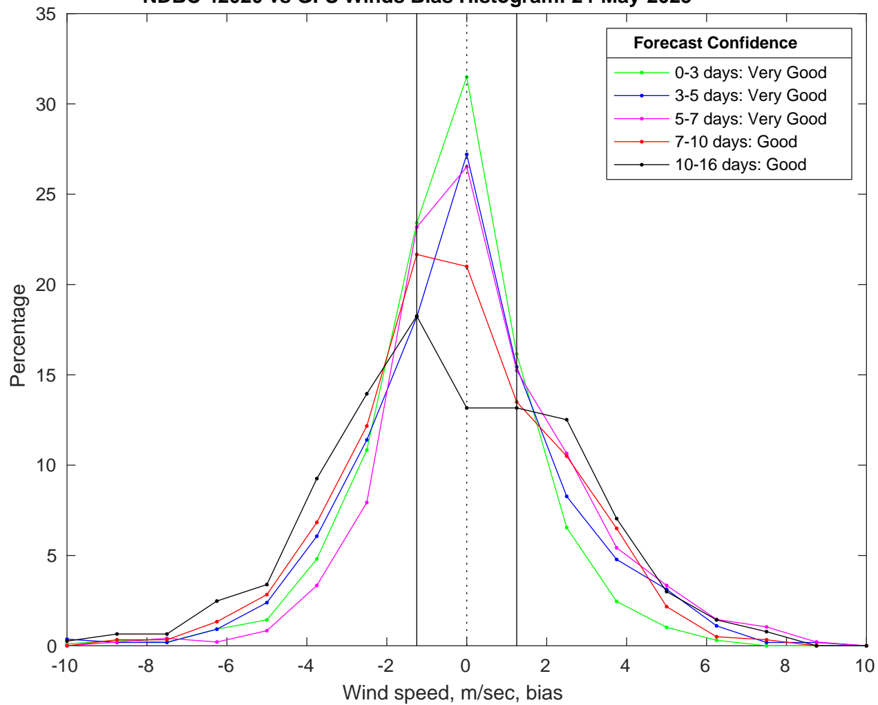
NDBC 42020 vs GFS Winds Bias Histogram: 24-May-2025
