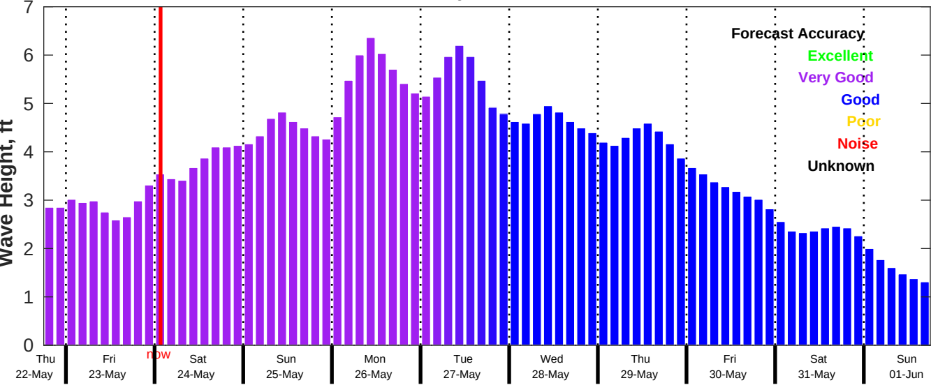
CMEMS Wave Forecast for NDBC 42020 from 22-May-2025 18:00:00 to 01-Jun-2025 18:00:00
