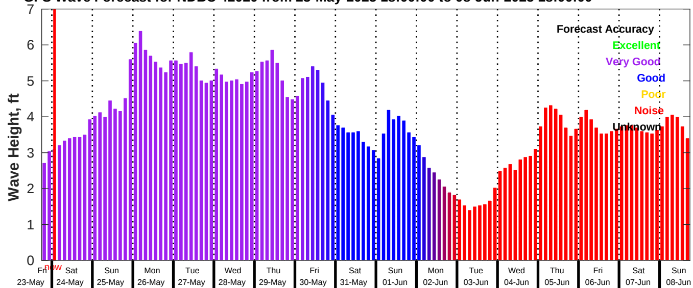
GFS Wave Forecast for NDBC 42020 from 23-May-2025 18:00:00 to 08-Jun-2025 18:00:00
