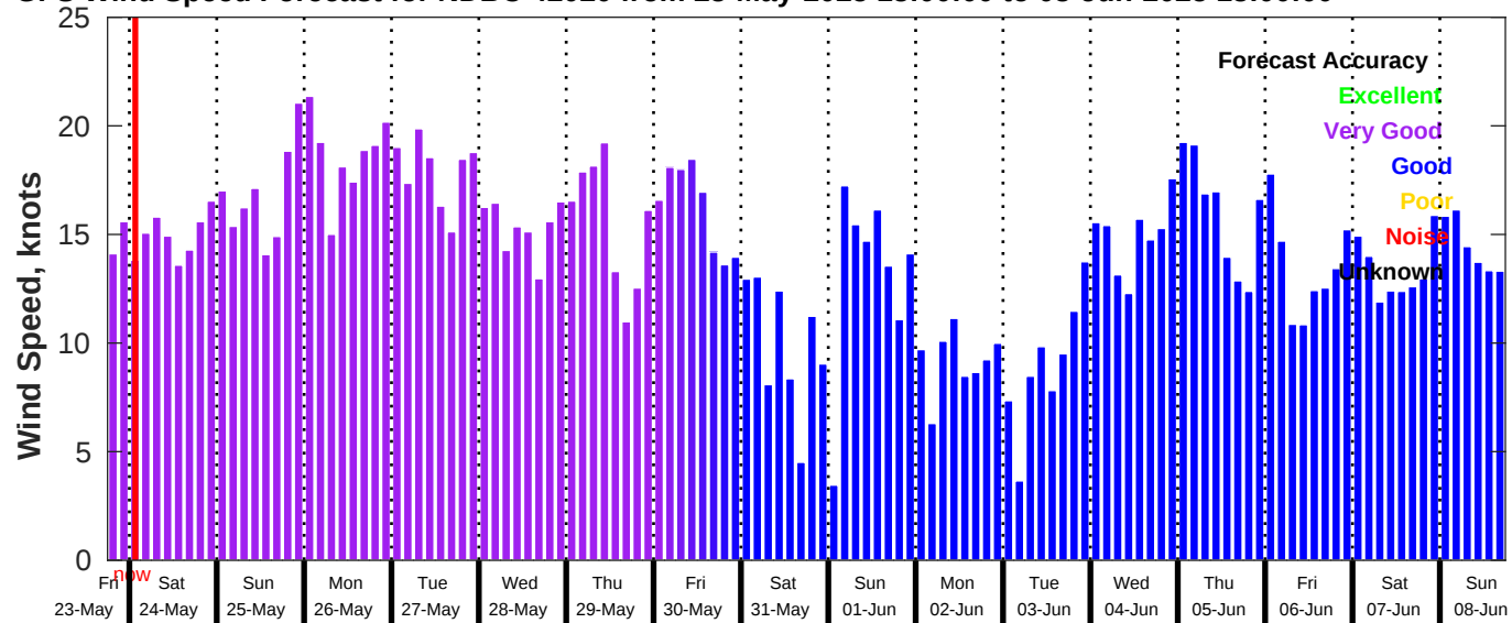
GFS Wind Speed Forecast for NDBC 42020 from 23-May-2025 18:00:00 to 08-Jun-2025 18:00:00
