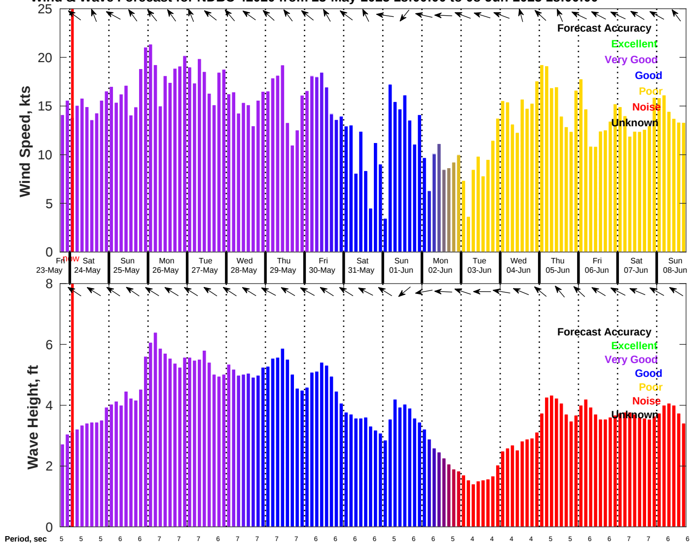
Wind & Wave Forecast for NDBC 42020 from 23-May-2025 18:00:00 to 08-Jun-2025 18:00:00
