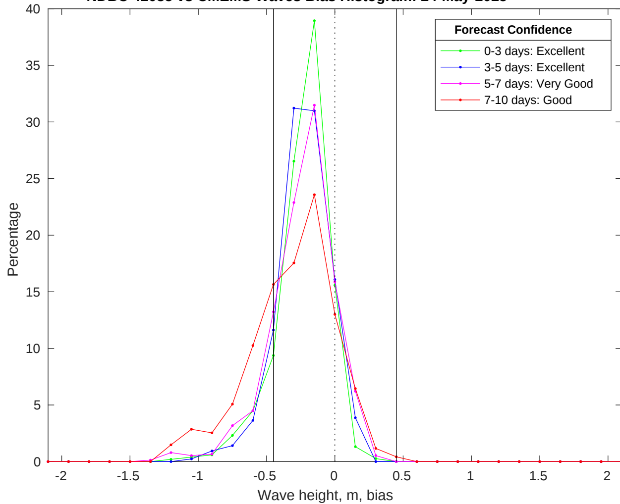
NDBC 42035 vs CMEMS Waves Bias Histogram: 24-May-2025
