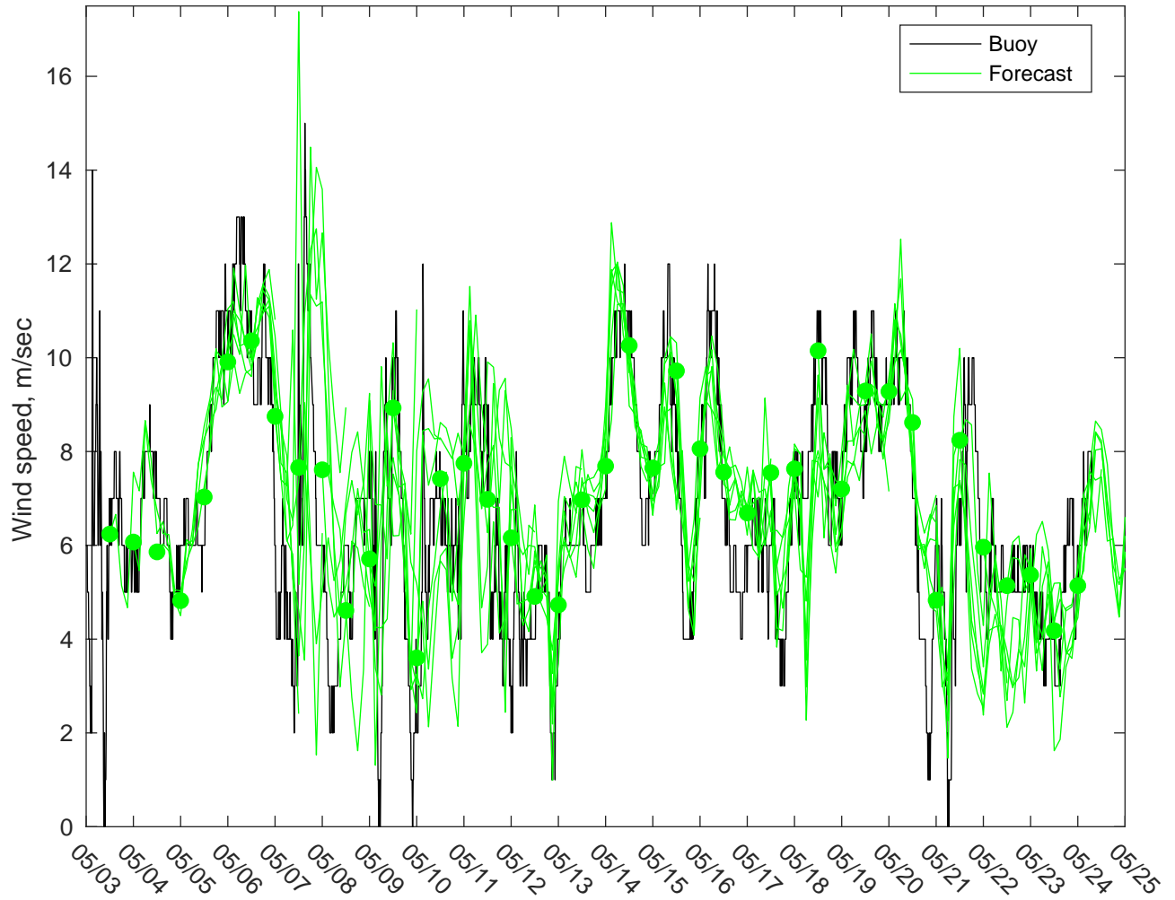
NDBC 42035 vs GFS Winds: 0 to 3 day forecast
